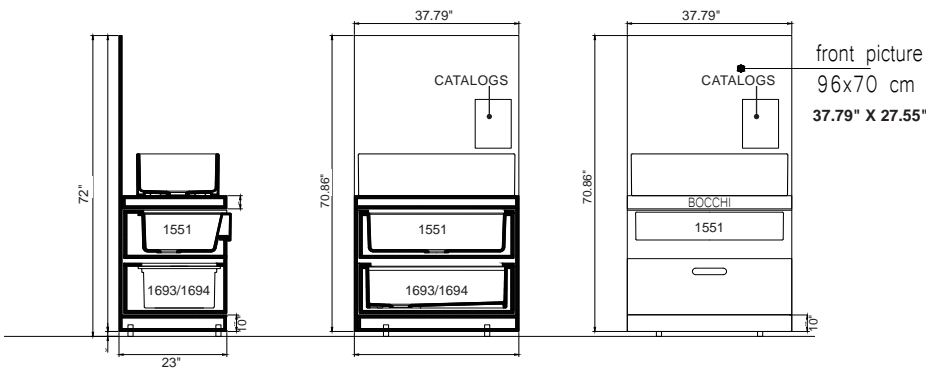
C-01 Fireclay Display Unit: Fits 3 sinks, you choose your colors... A) choose an apron sink of your choice for the top; B) a Nuova Pro short-front apron sink (1551); and C) a showroom exclusive Sotto Step-Rim undermount (1693 or 1694).
