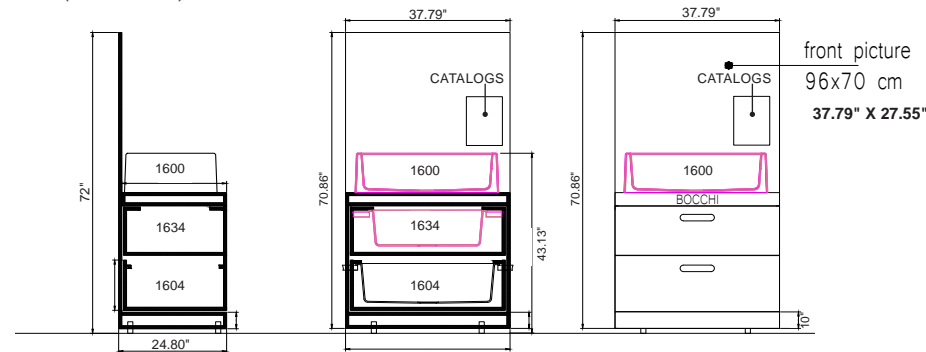
C-02 Granite Display Unit: Fits 3 sinks, you choose your colors... A) Arona Granite Apron Sink (1600) on the top (or a fireclay apron of your choice); B) Campino Uno (1634) in the center drawer; and C) larger Campino Uno (1604) in the bottom drawer.
